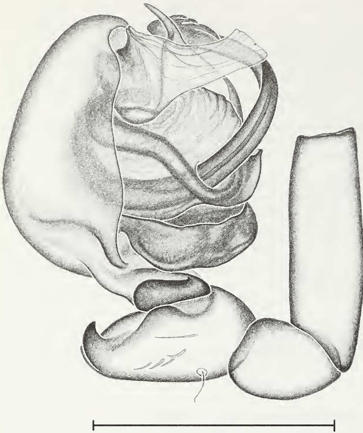
Fig. 1: Male left palp, retrolateral view, hairs omitted. Specimen from Siggenthal (Aarau, Switzerland). Scale: 200 \mu m.
